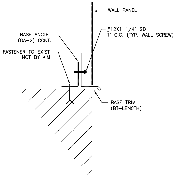
DETAIL B
