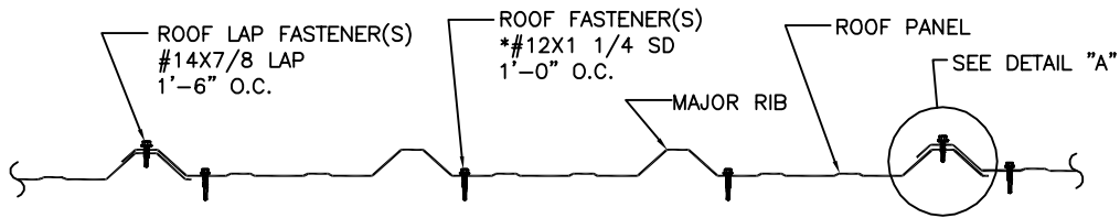
TYPICAL FASTENER LAYOUT AT INTERMEDIATE PURLINS
