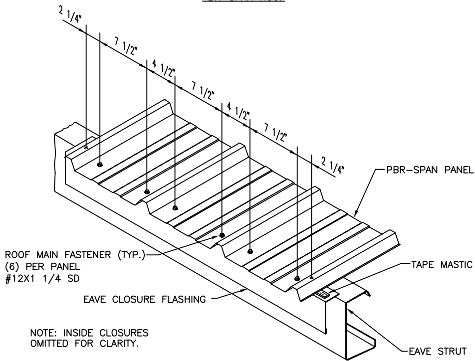
FASTENER INSTALLATION AT EAVE STRUT
