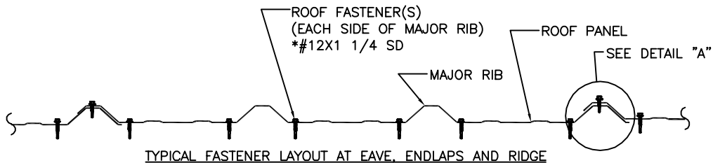
TYPICAL FASTENER LAYOUT AT EAVE, ENDLAPS AND RIDGE
