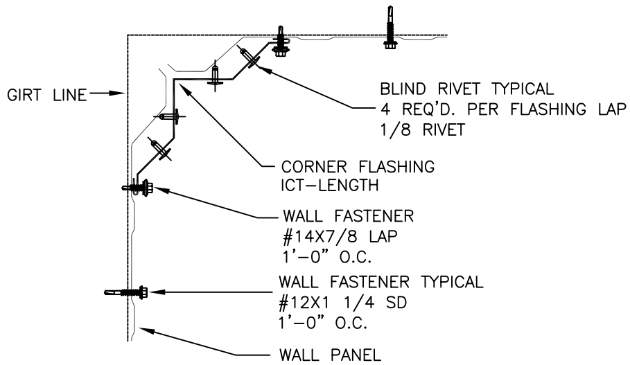
CORNER FLASHING DETAIL (INSIDE)
