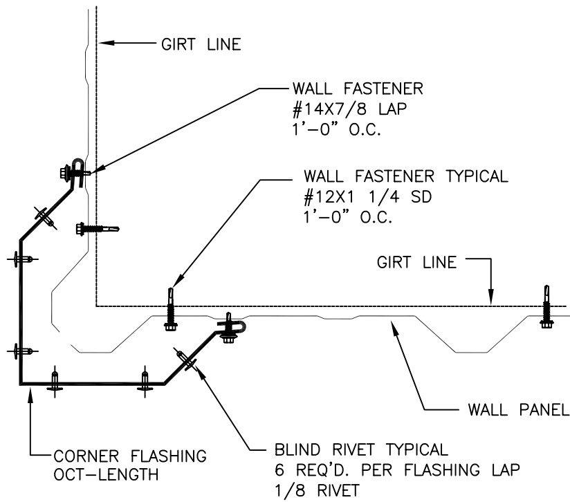
CORNER FLASHING DETAIL (OUTSIDE)
