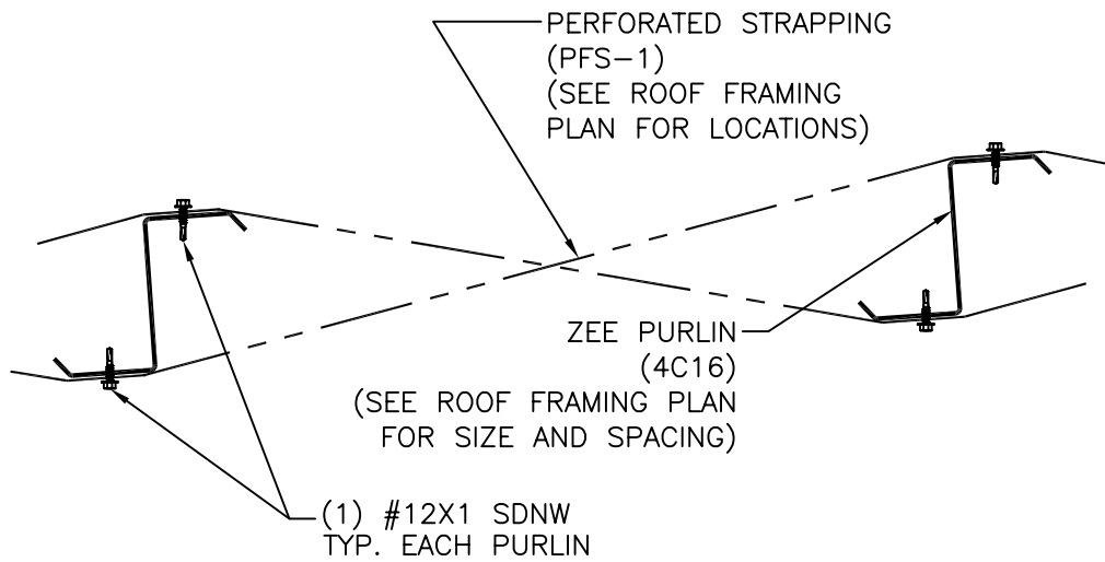
AT INTERMEDIATE ZEE PURLIN
