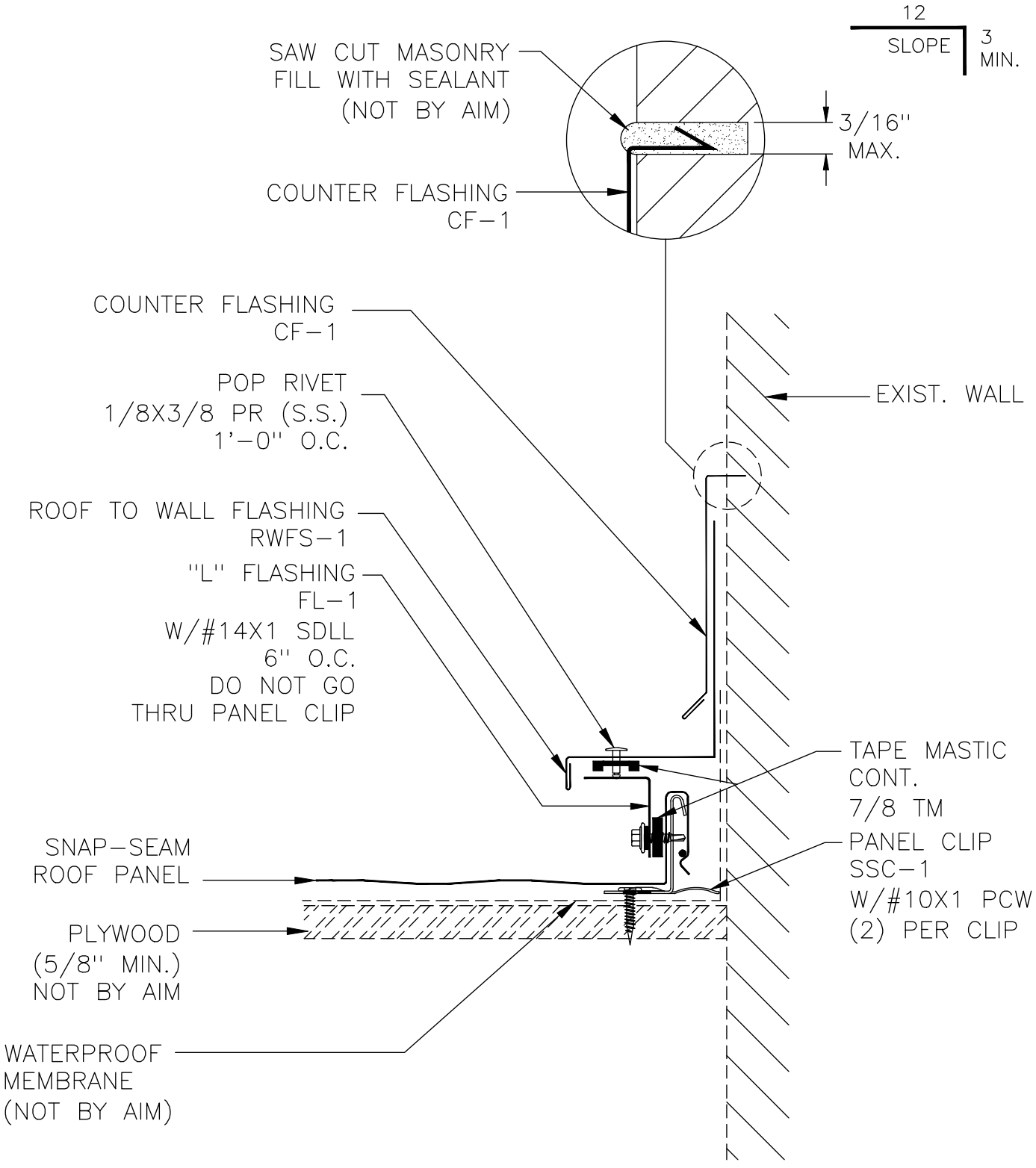
GABLE ROOF TO WALL ON WOOD (STARTING) FOR SNAP-SEAM PANELS (FLOATING CONDITION)
