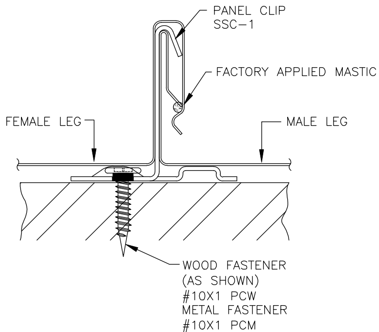
SECTION THROUGH PANEL AT CLIP
